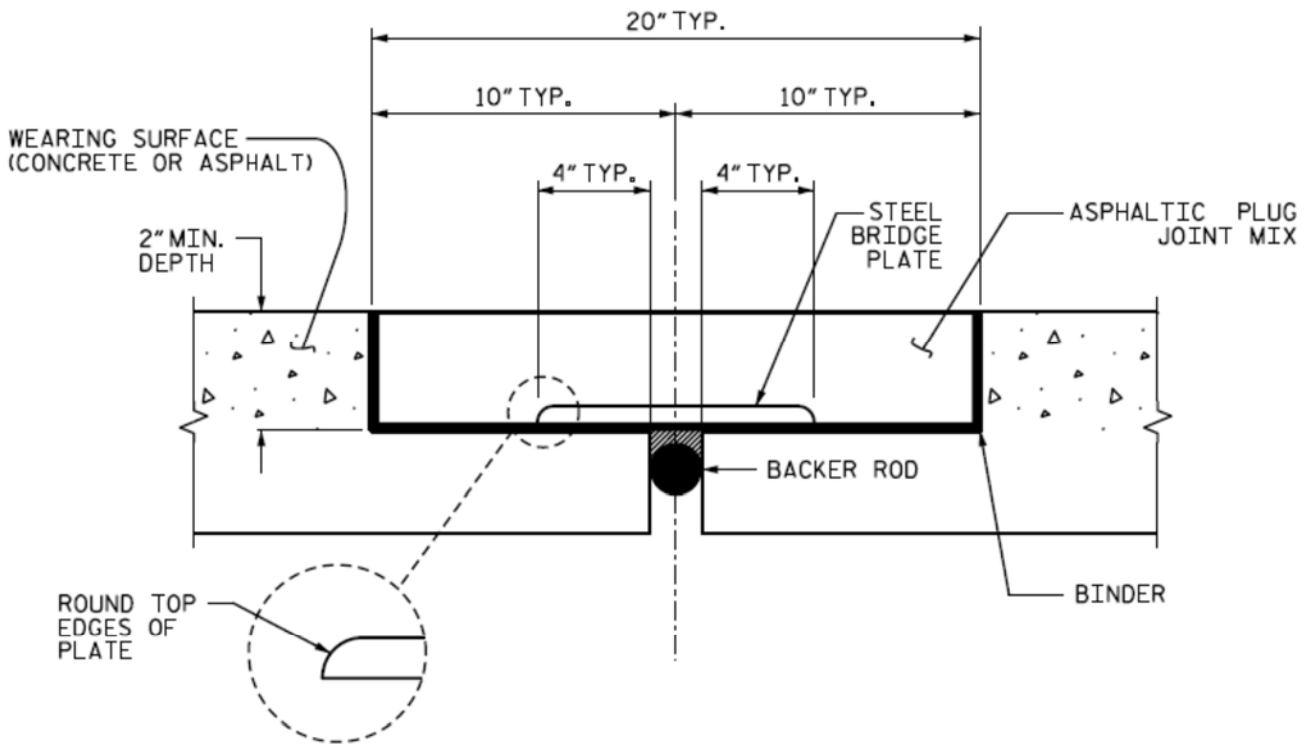
ASPHALTIC PLUG JOINT DETAIL
